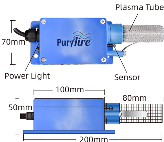
SG-Mini-5A Dimensions
