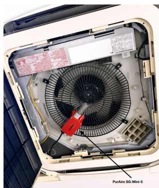
Cassette Installation
