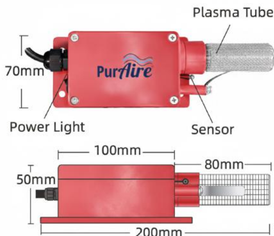
SG-Mini-5A Dimensions
